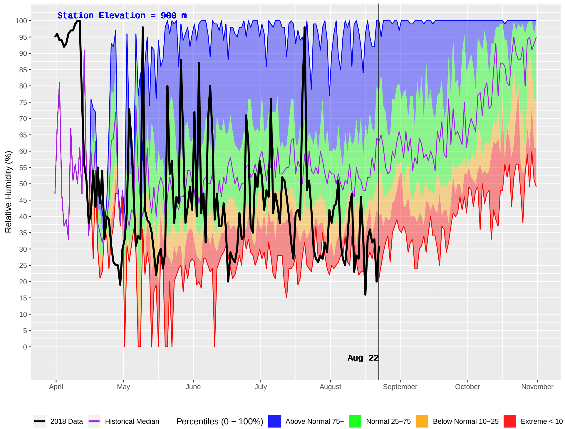
UPPER FULTON (169) : Historical (1986–2016) and Current (2018) Daily Relative Humidity
