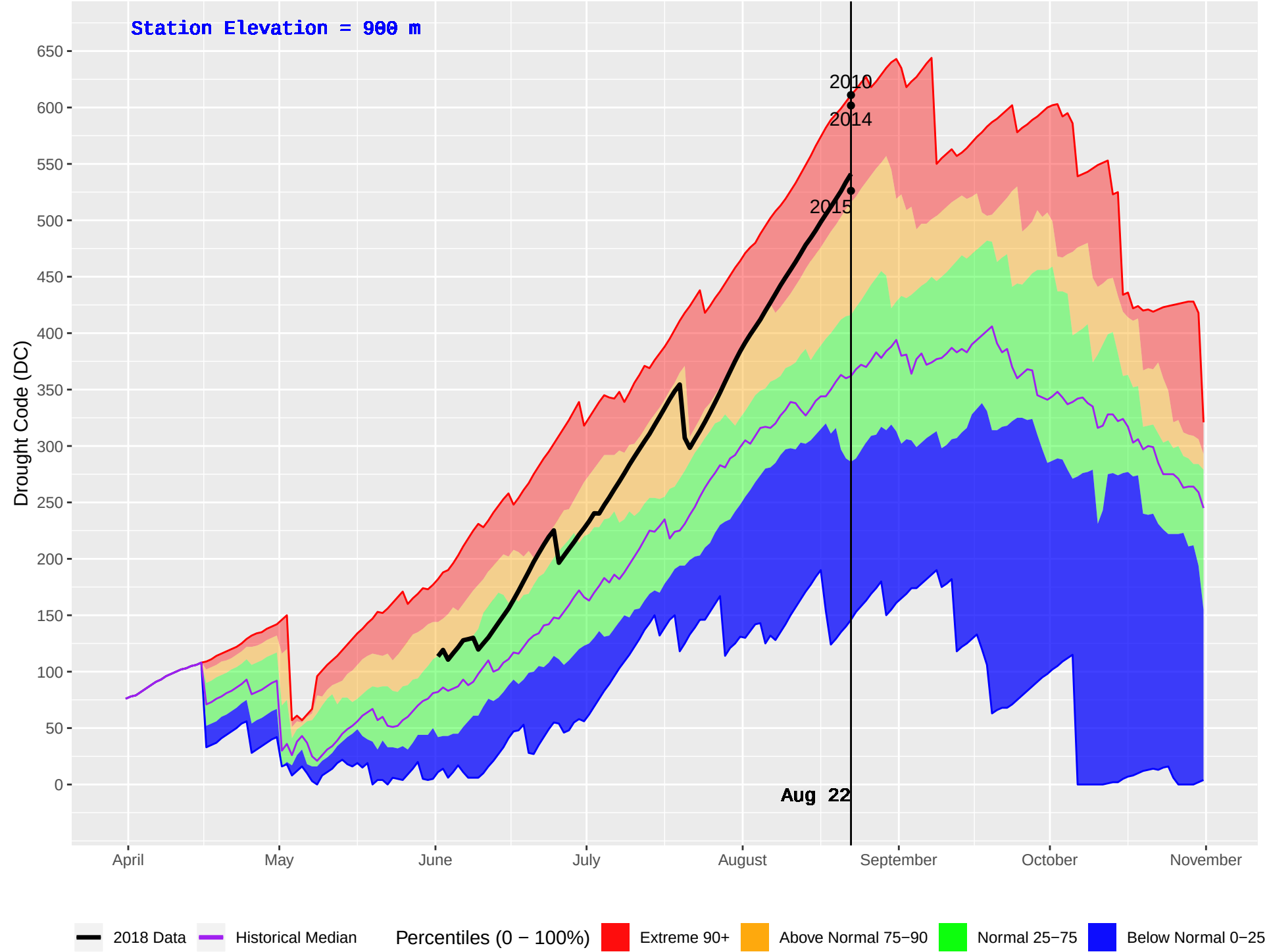
UPPER FULTON (169) : Historical (1986–2016) and Current (2018) Daily Drought Code (DC)
