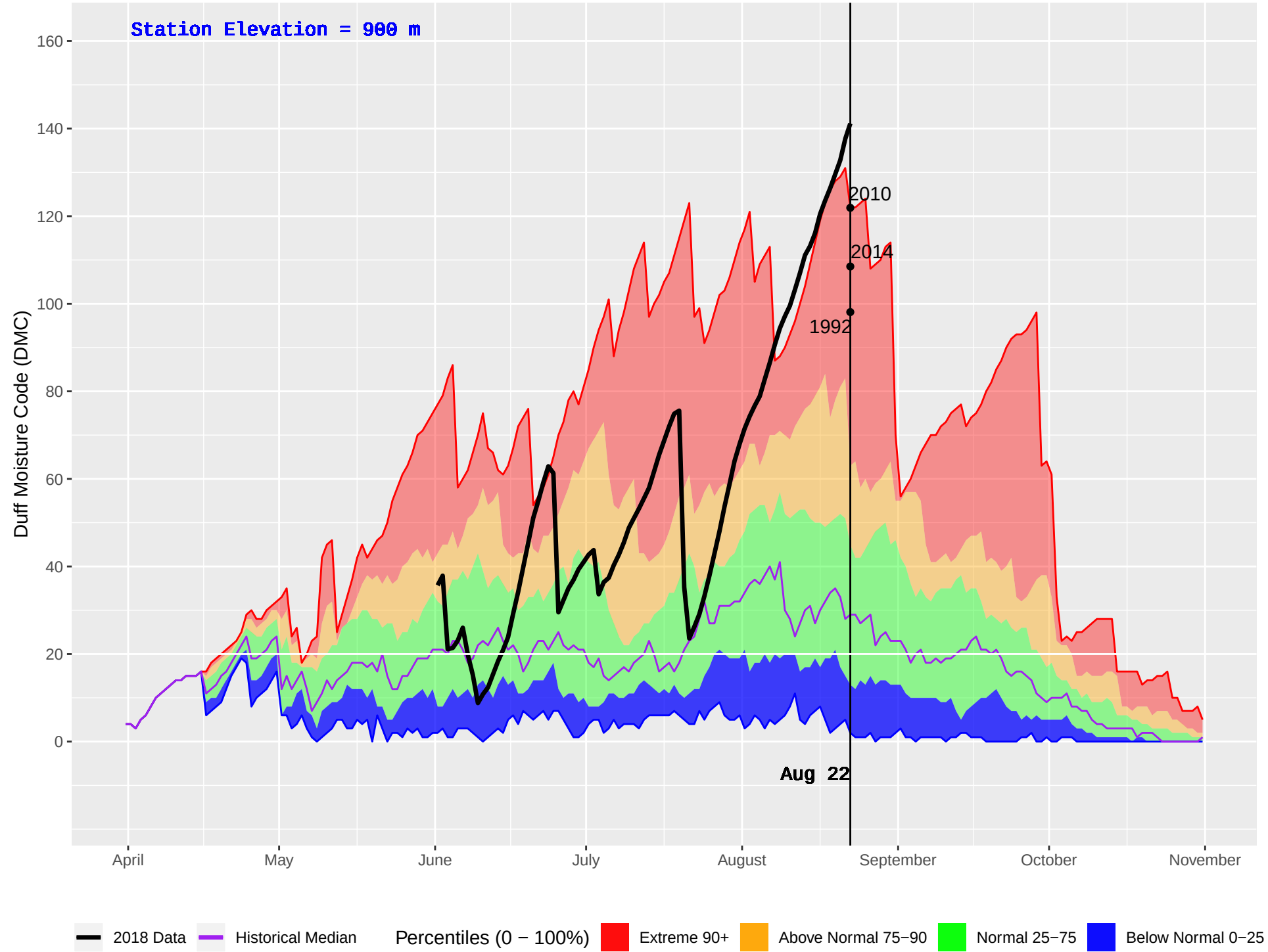
UPPER FULTON (169) : Historical (1986–2016) and Current (2018) Daily Duff Moisture Code (DMC)
