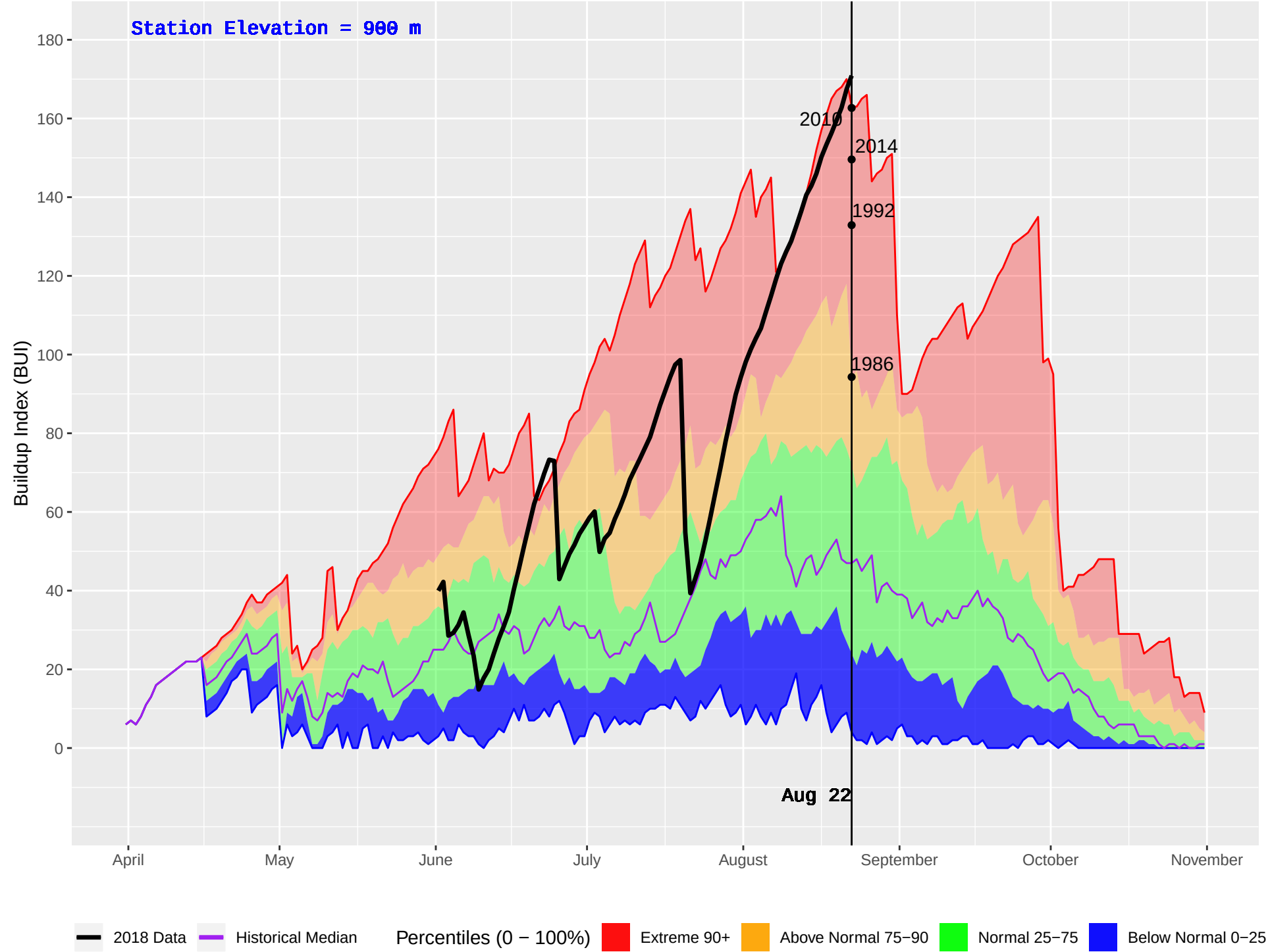
UPPER FULTON (169) : Historical (1986–2016) and Current (2018) Daily Buildup Index (BUI)
