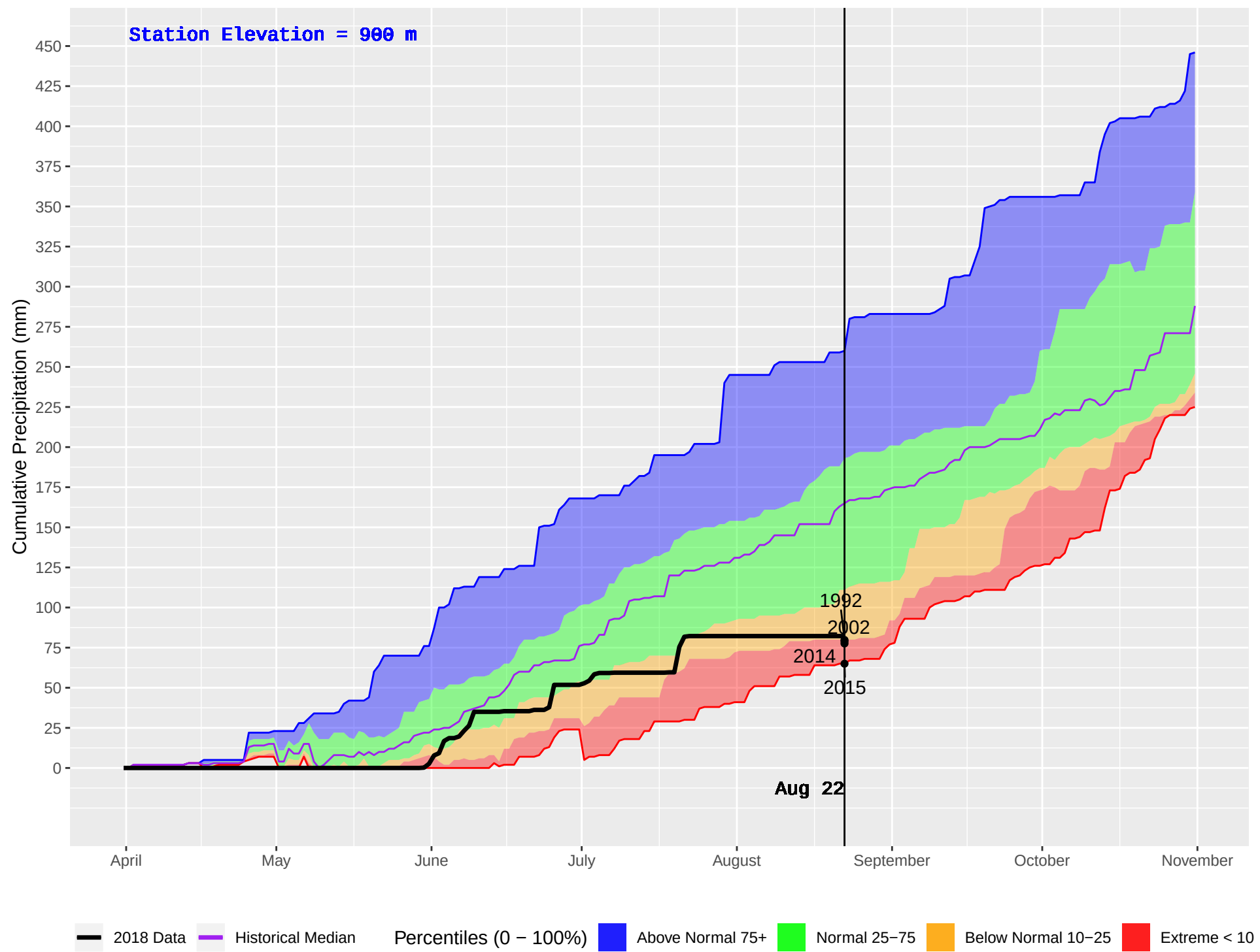
UPPER FULTON (169) : Historical (1986–2016) and Current (2018) Daily Cumulative Precipitation
