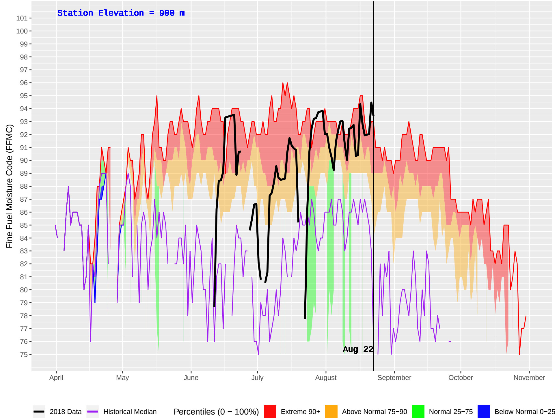
UPPER FULTON (169) : Historical (1986–2016) and Current (2018) Daily Fine Fuel Moisture Code (FFMC)
